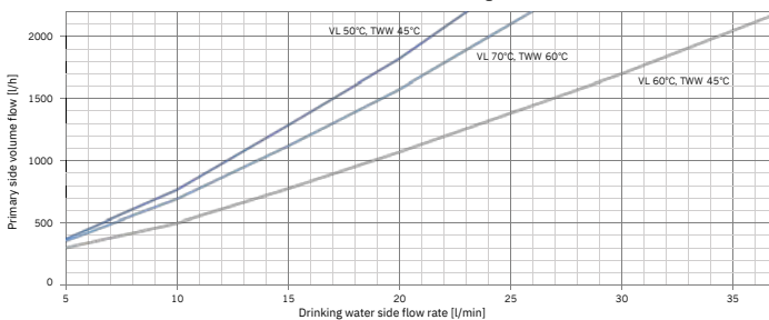
Volume flow on the primary side at different supply temperatures for domestic hot water heating
