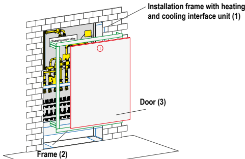
Schematic diagram - Flush-mounted
